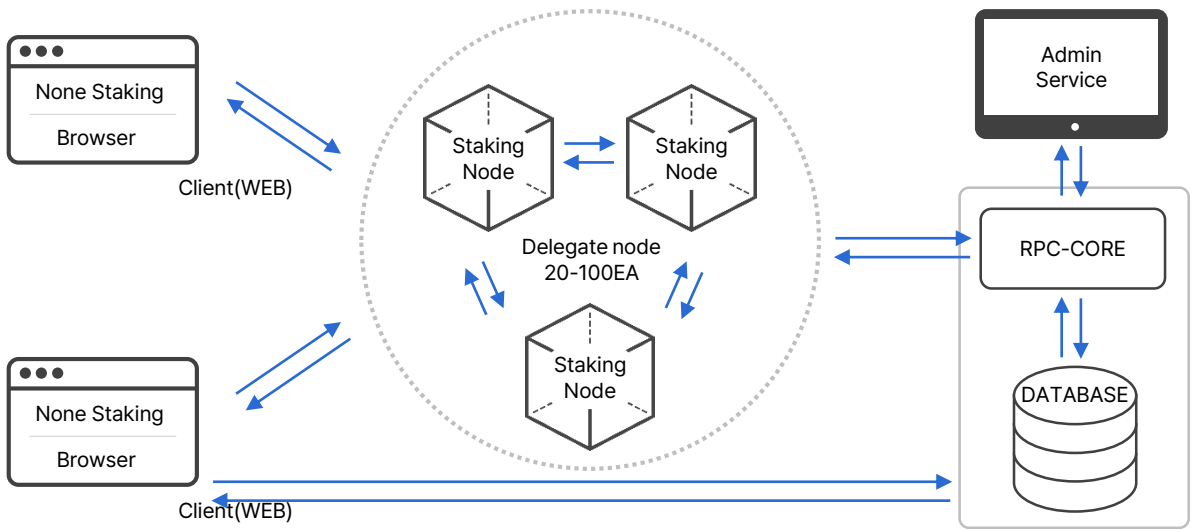
<Figure1. Structure of RYSEN blockchain system>
